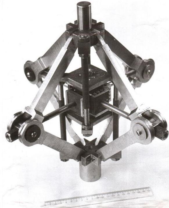
Fig.1. Device for three axial tension
