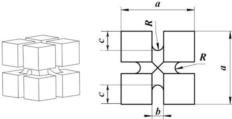
Fig. 2. The sample for the three axial tension
